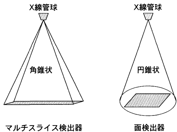
Fig. 2. Two types of X-ray beam
