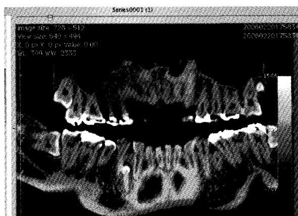
Fig. 9. Curved MPR
